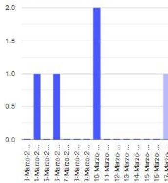
Volcanotectonicos
